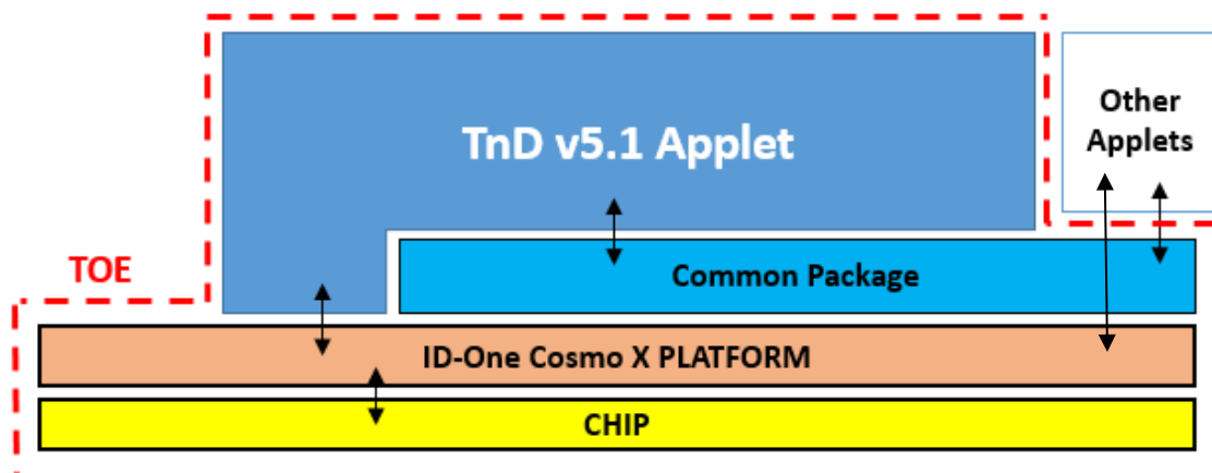
Figure 2 TOE's logical architecture
